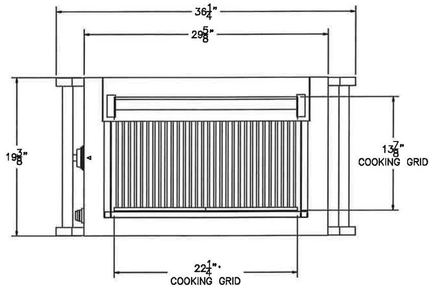
TOP VIEW (SHOWN WITH HOOD OPEN)
