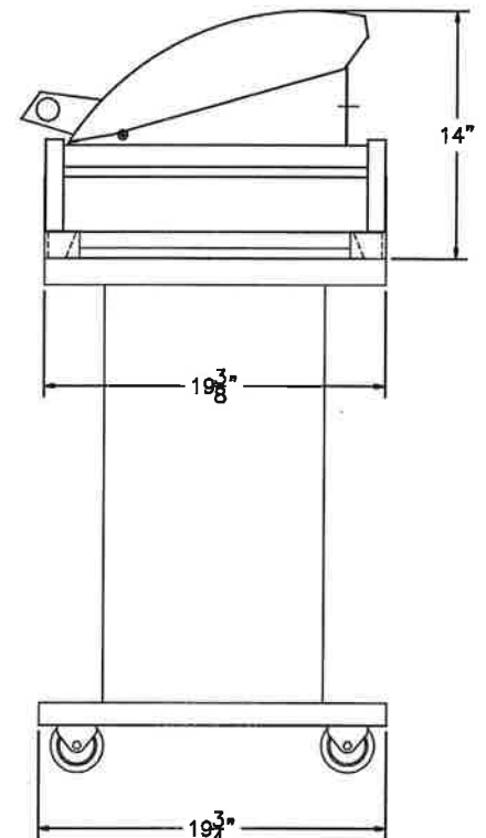
END VIEW
