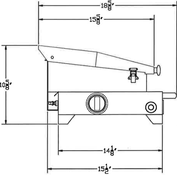
END VIEW
